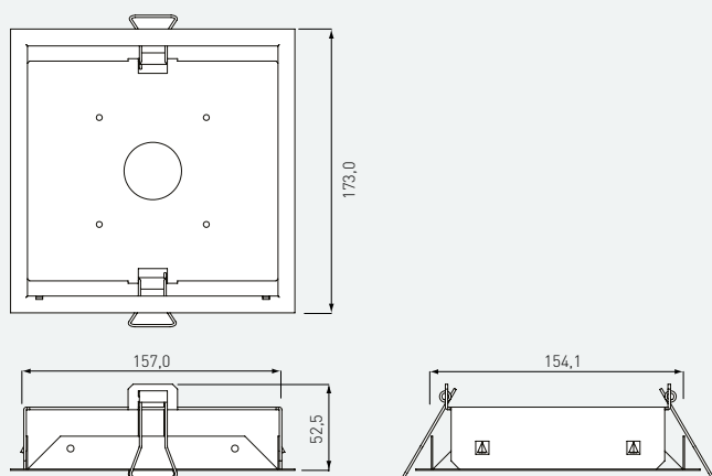
K1RH1 - mounting frame
