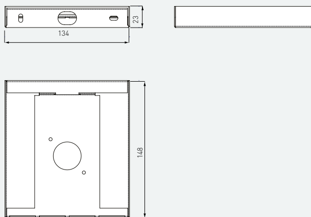
K1RH2 - right angle wall bracket
